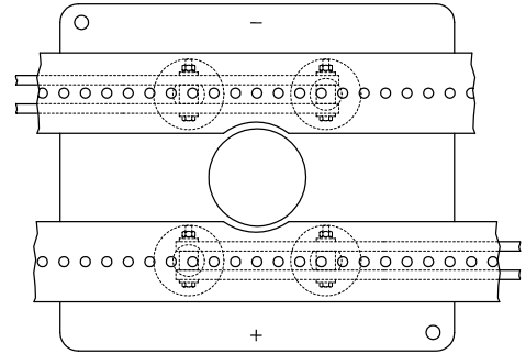
Top view of covers over the battery terminals
