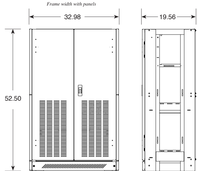
Front view and side view dimensions of frame with panels all measurements shown in inches
