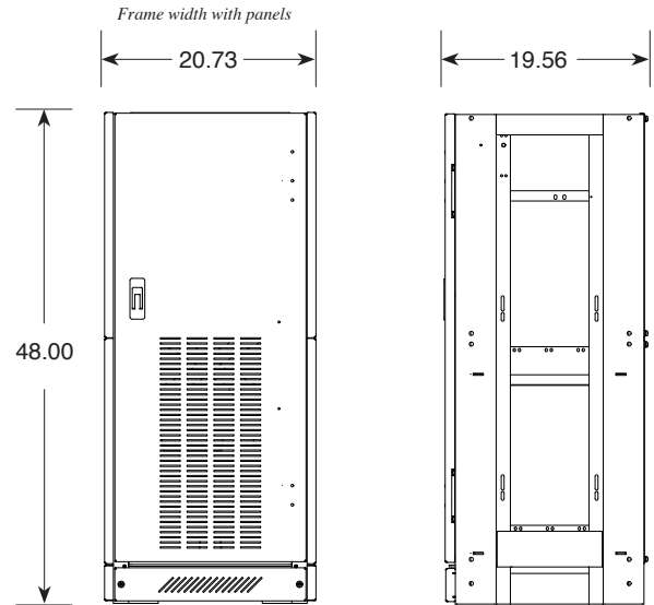
Front view and side view dimensions of frame with panels all measurements shown in inches
