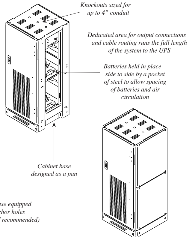
Isometric views shown with and without side panels
